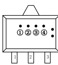
SOT89-3L (Top View)
