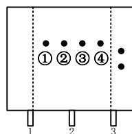
TO-92S (Front View)
