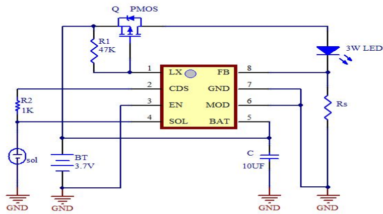
LED 电流=90mV/Rs
